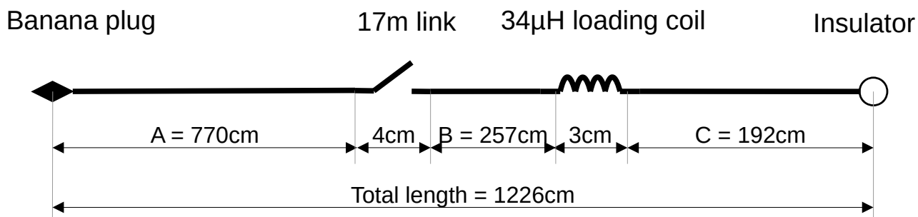
Figure 36: The compact antenna dimensions
