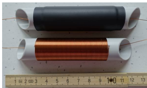
Figure 34: Building the 80-meter-band loading coil
