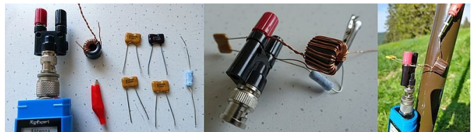
Figure 2: Coupler experiments
